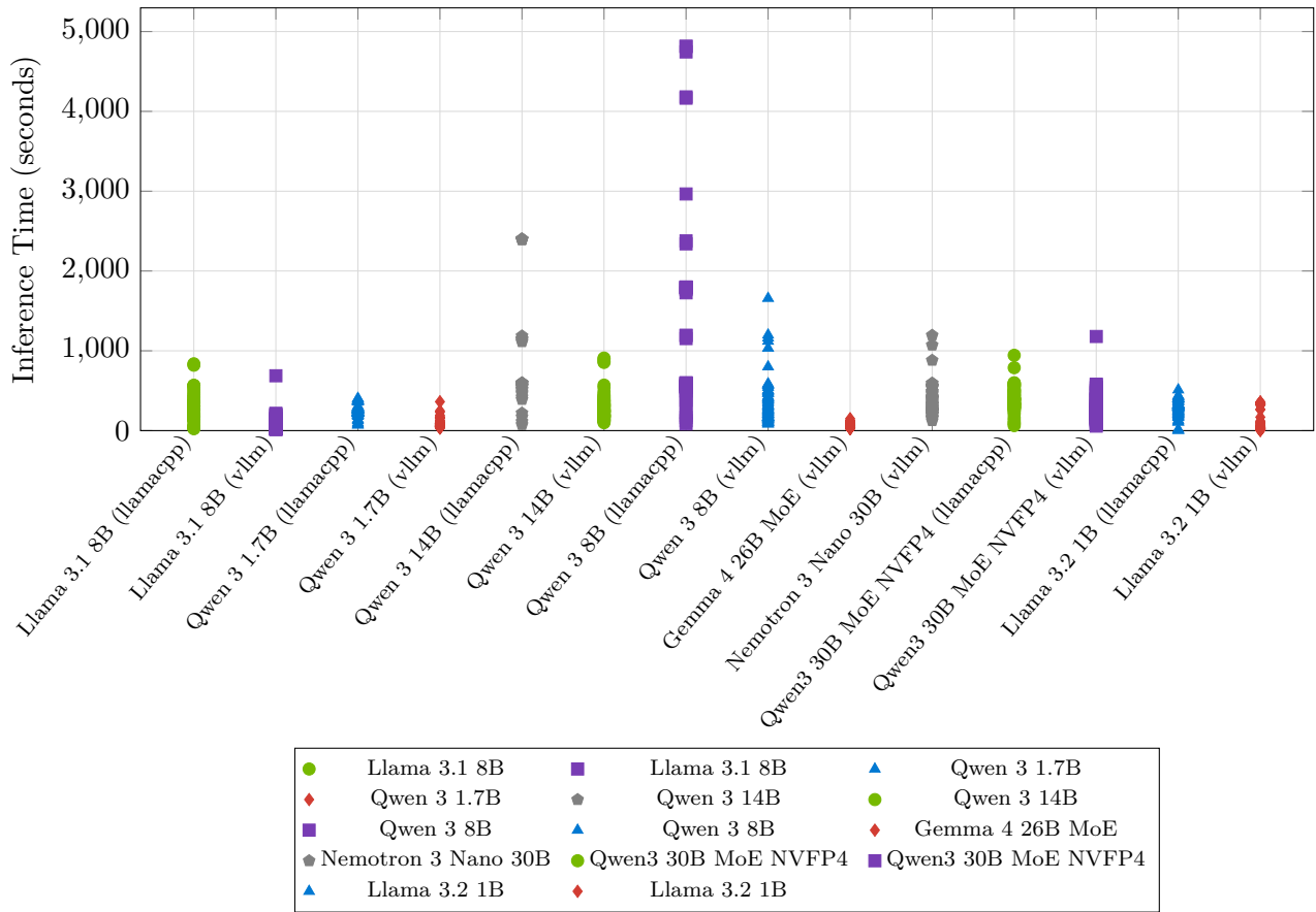
Figure 3: Per-sample inference time scatter plot. Each point represents one evaluation sample. Variation reflects differences in output length and complexity.
