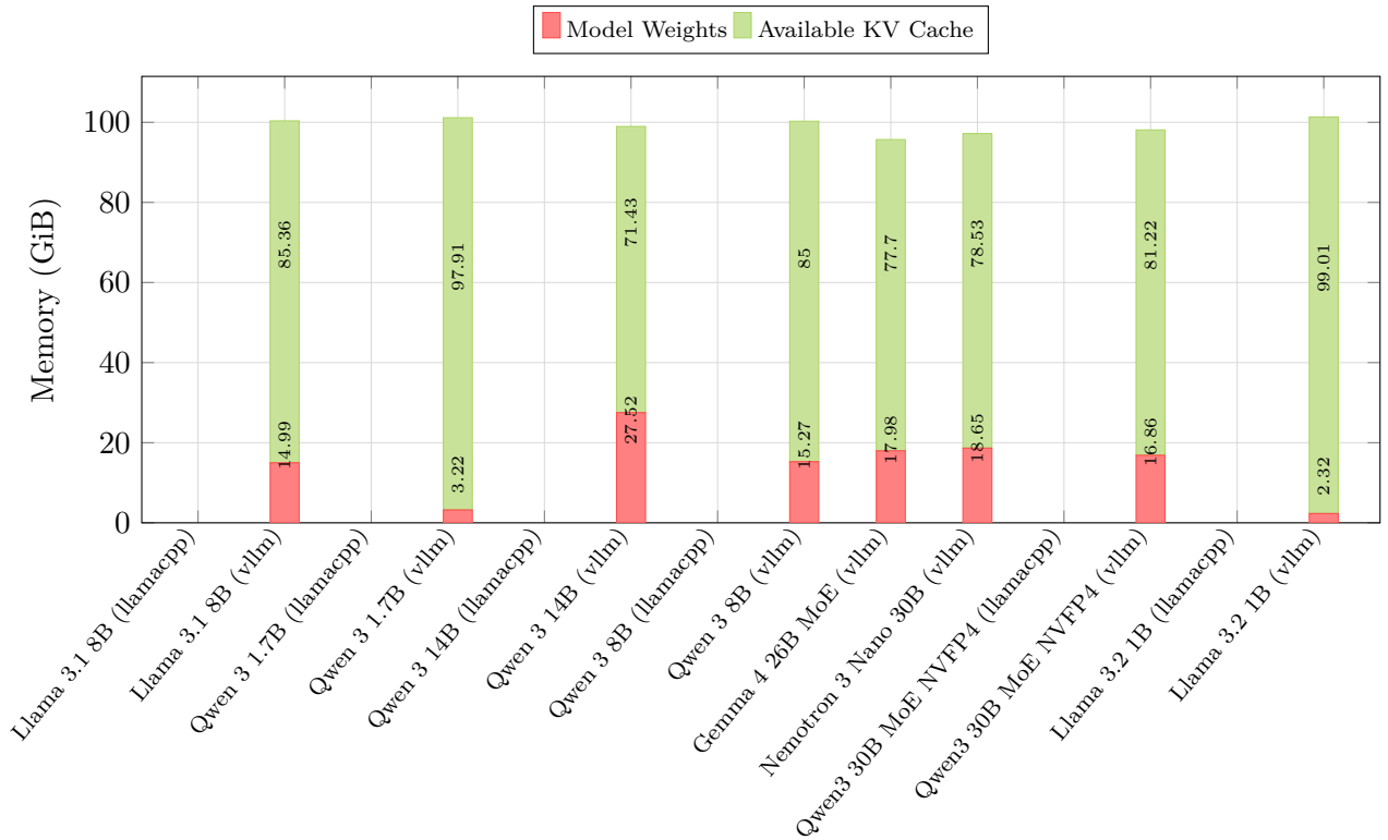
Figure 5: GPU memory allocation per model. Smaller model footprints leave more memory for KV cache, enabling higher concurrency and longer context windows. Total RAM: 122 GiB.
